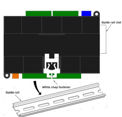
Figure 4: Pull down the white snap of the product and insert it into the rail strip. Then press the white snap upwards as shown in the figure to fix it.
