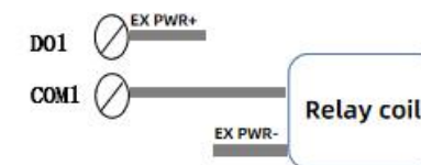
Figure 2: Digital Output Wiring Diagram
